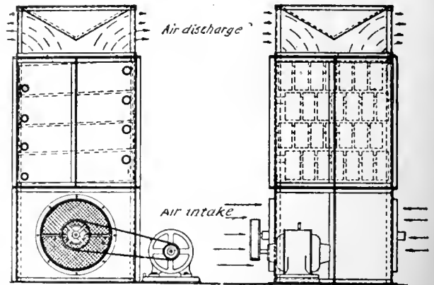
FIG. 10. TYPICAL UNIT HEATER FOR PLACING ON THE FLOOR
